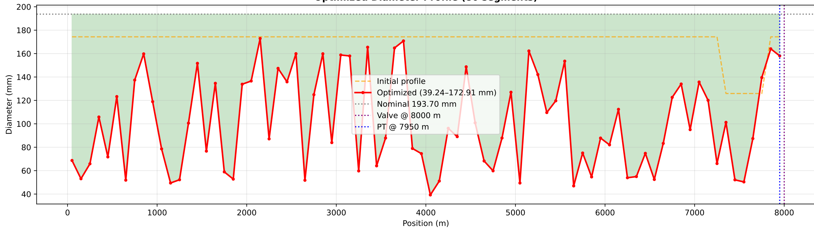
Optimized Diameter Profile (80 segments)
