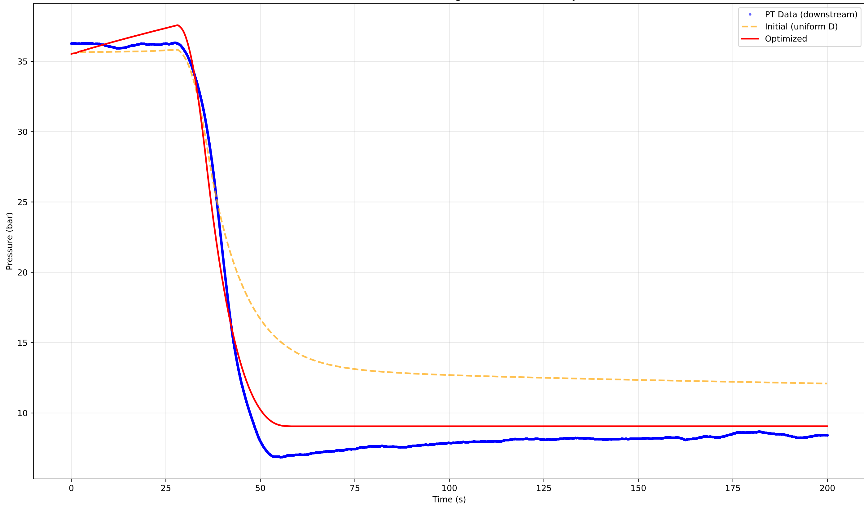
Downstream Pressure Match — Segmented Diameter Optimization
